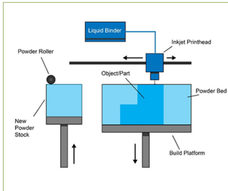
Image 1: Binder jetting
