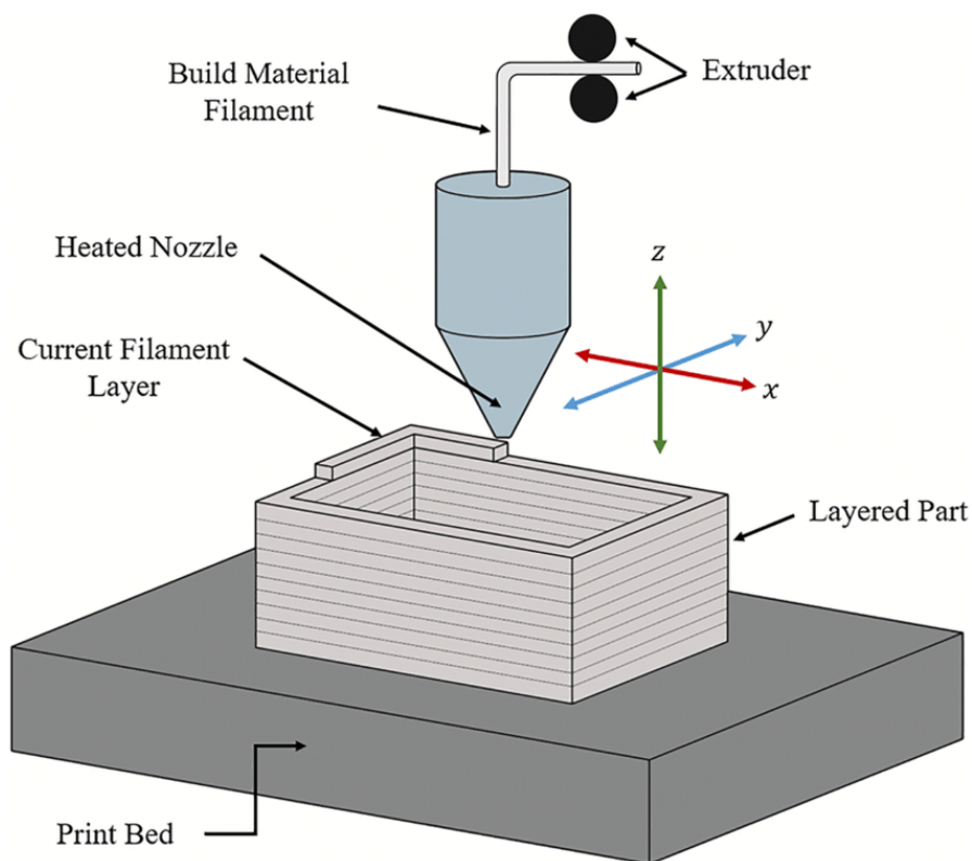
Image 2: Materials extrusion
