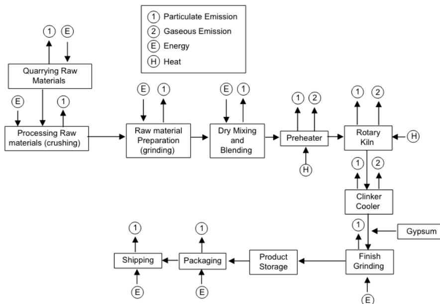
Image 10: Portland cement diagram (source: Huntzinger & Eatmon, 2009)
