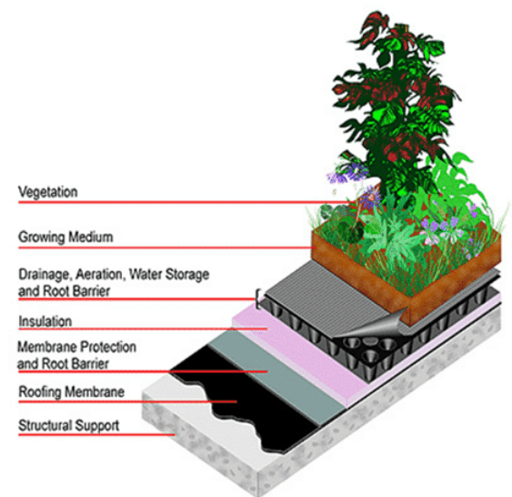
Image 17: Green roof layers (source: Manso, Teotónio, Silva & Oliveira Cruz, 2021)
